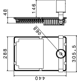
Integrated pole-top mounting
