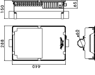
Horizontal pole mounting
