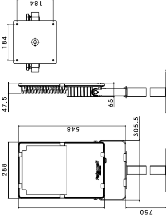
Wall mounting with projecting bracket
