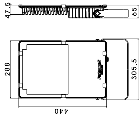
Wall mounting with bracket
