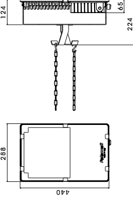
Adjustable double chain suspension
