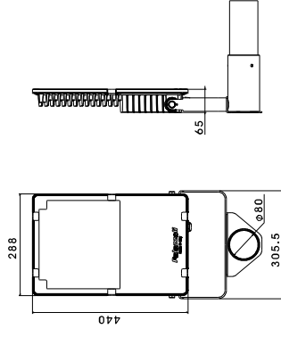
Pole-top mounting with accessories
